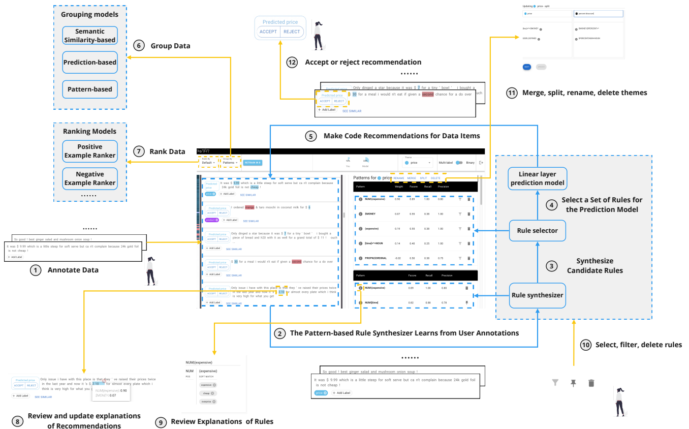
Figure 2: The system architecture of PaTAT: While (1) the user starts annotating data on the left panel, (2) PaTAT learns patterns from the user’s annotations by (3) synthesizing rules over parts of speech, literal words, word lemmas, soft matches, entity types, and wild cards. (4) PaTAT selects a small set of rules that can capture the broadest of positive annotations and trains a linear layer model. Then PaTAT (5) recommends codes for data items in the left panel based on that linear model over patterns. The user has the option to group (6) and rank (7) data based on different strategies. The user can give feedback to the model by reviewing and updating recommendations (8), reviewing and updating rules (9), and selecting and removing rules (10). The user can iteratively update the codebook (11), and make annotations by accepting/rejecting recommendations (12) Yellow lines represent users’ interaction, while blue lines represent PaTAT’s information flow.
