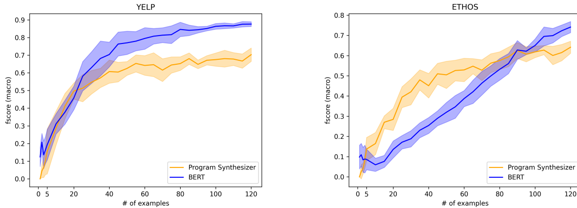
Figure 4: The change in prediction performance (F1-Score) of the BERT model and PaTAT’s pattern synthesizer model over the number of training examples in YELP and ETHOS datasets. The shades represent the standard error of the mean F1-score.
